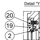
Detail "Y"
