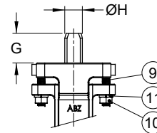
2" thru 8" Stem
