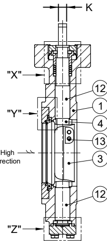
Section View
